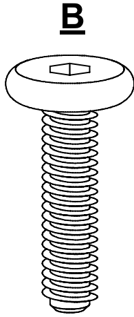
B M6*25 4 PCS
